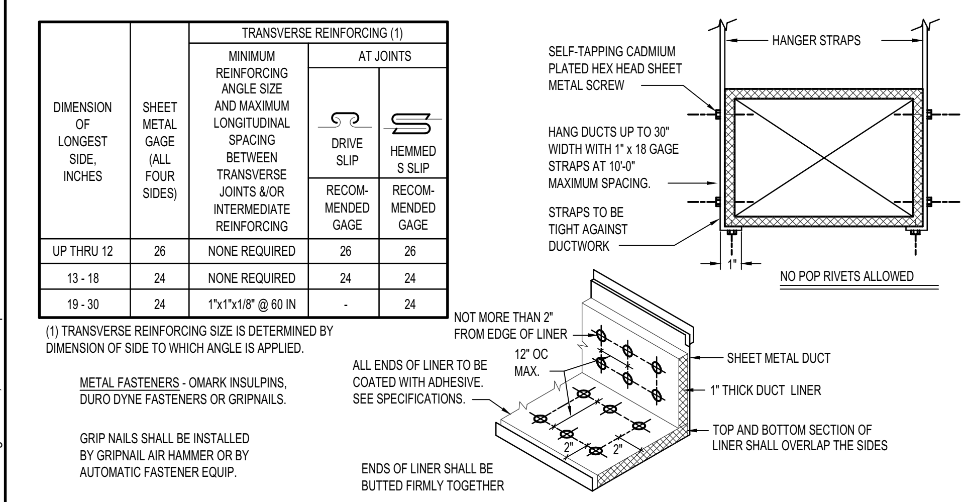
N | DUCT CONSTRUCTION AND HANGER DETAILS NO SCALE
