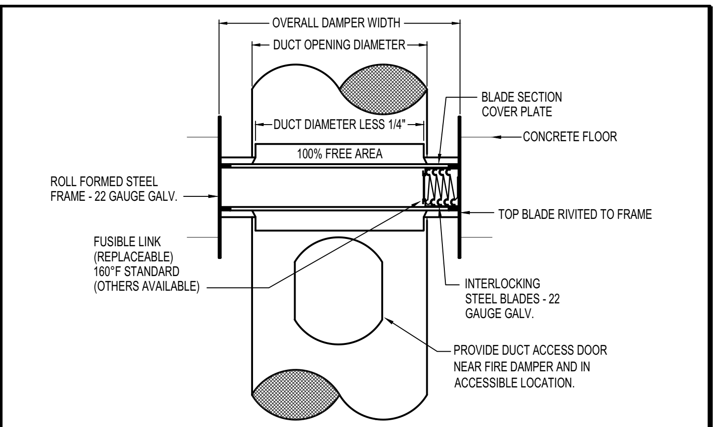
D | FIRE DAMPER DETAIL THRU FLOOR NO SCALE
