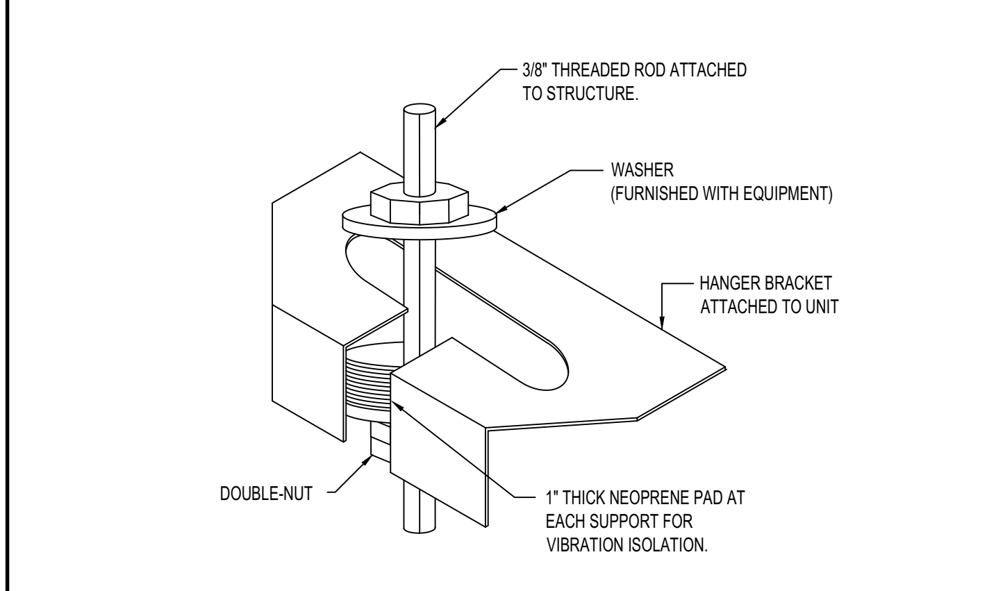
E | EQUIPMENT HANGER DETAIL NO SCALE
