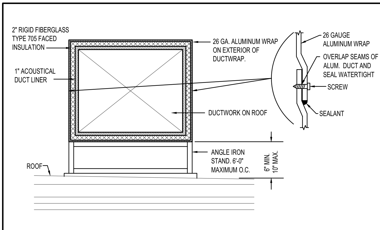
A | EXPOSED DUCT INSULATION NO SCALE
