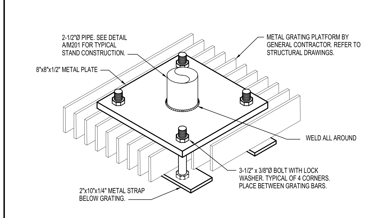
F | TANK STAND ANCHOR DETAIL NO SCALE
