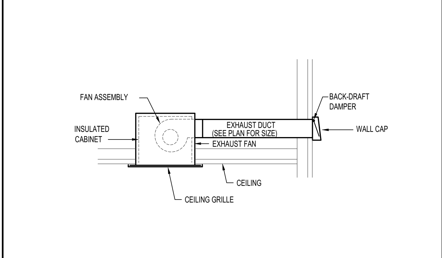
G | EXHAUST FAN INSTALLATION DETAIL NO SCALE
