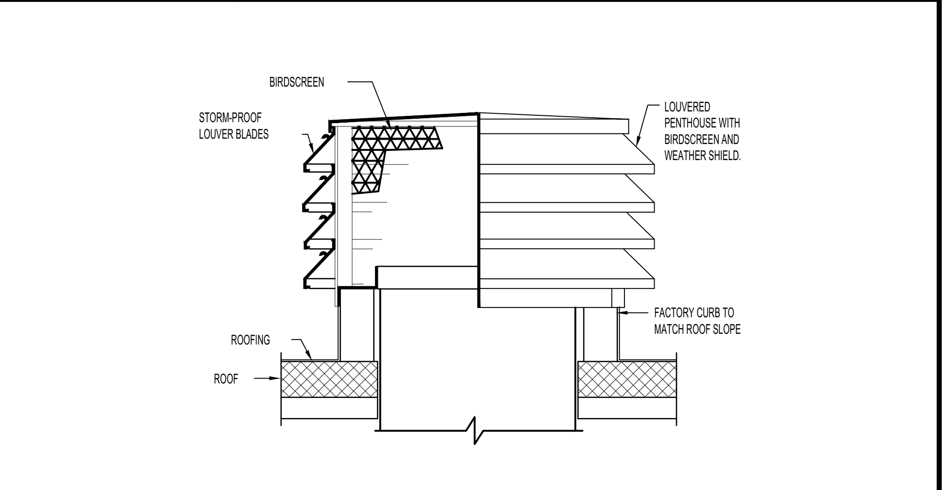
M | PENTHOUSE DETAIL NO SCALE
