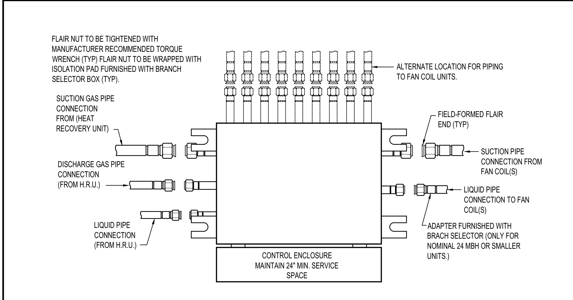
J | BRANCH SELECTOR BOX DETAIL NO SCALE
