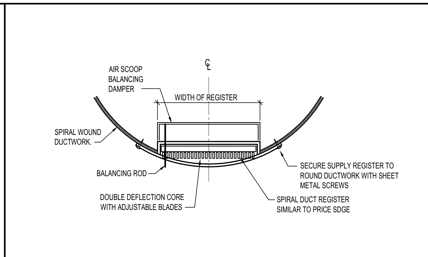
B | GRILLE IN ROUND DUCT DETAIL NO SCALE
