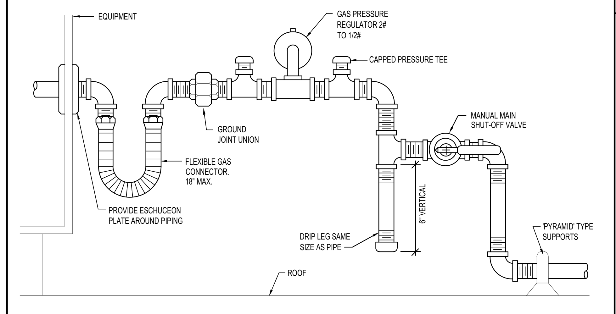
O | GAS LINE CONNECTION DETAIL NO SCALE
