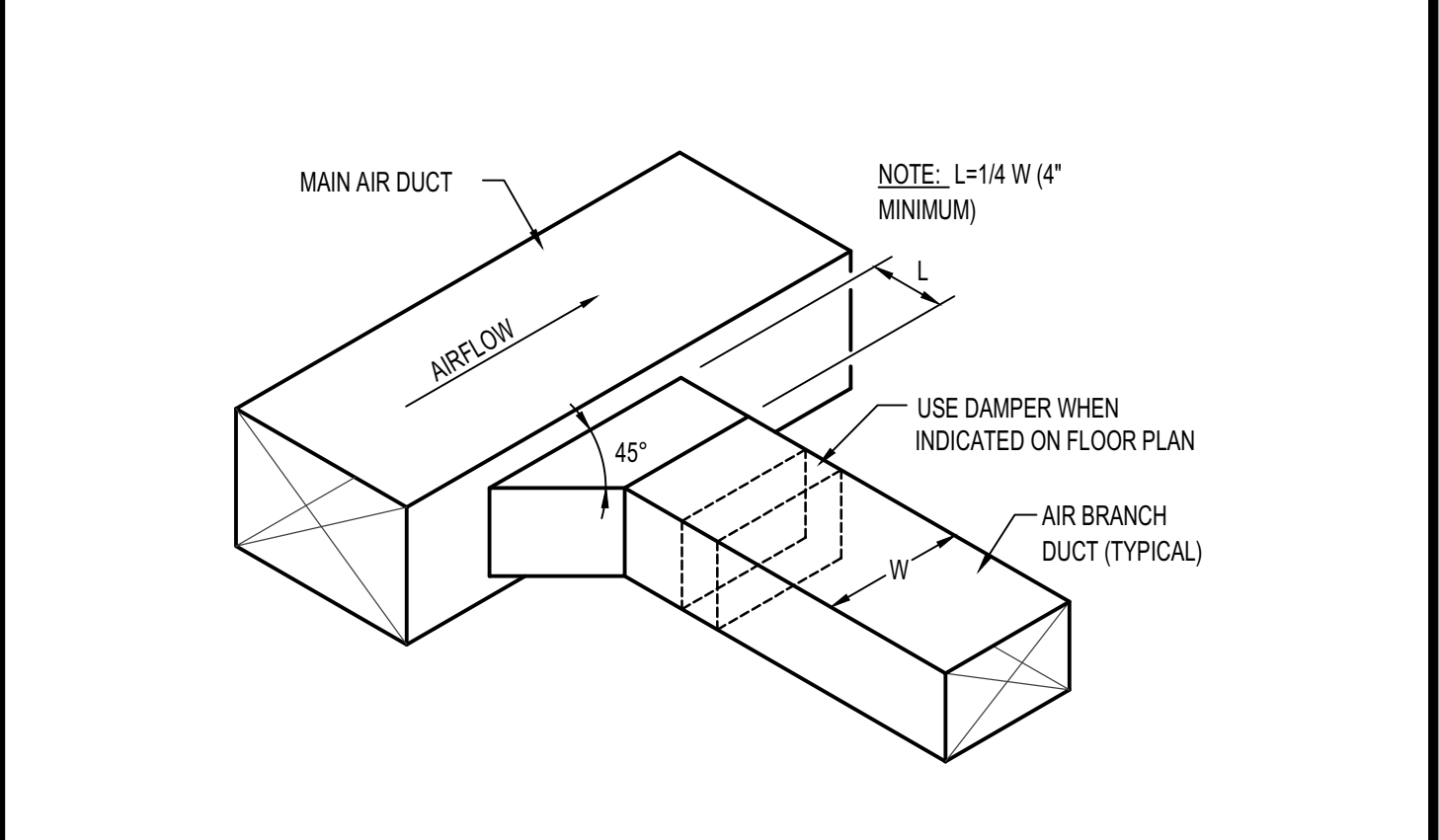
H | RECTANGULAR DUCT CONNECTION NO SCALE
