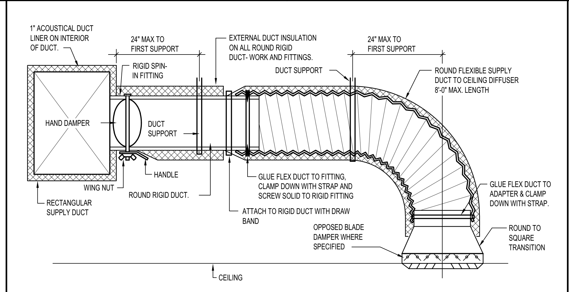
K | DIFFUSER INSTALLATION DETAIL NO SCALE
