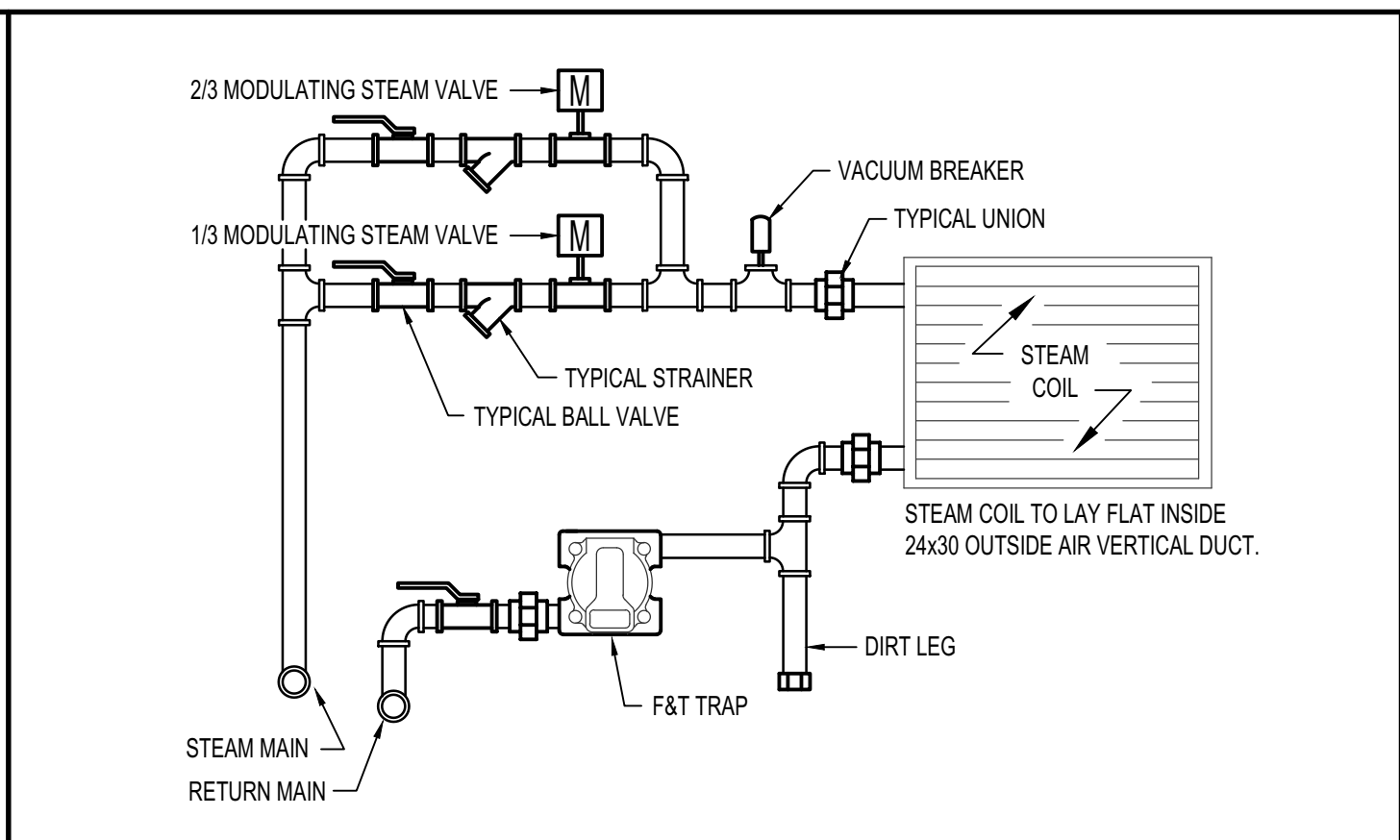
C | STEAM COIL PIPING DIAGRAM NO SCALE
